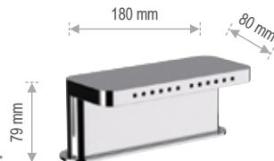
91 NCF Bocca bordo vasca con angoli arrotondati. Spout for deck bath/shower with rounded corners.
