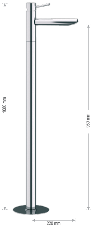
N 18 Miscelatore monocomando lavabo da terra. Single-lever mixer for floor mounting.
